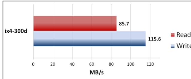
NASPT test: File copy to and from NAS using a single 1.15 GB file.
